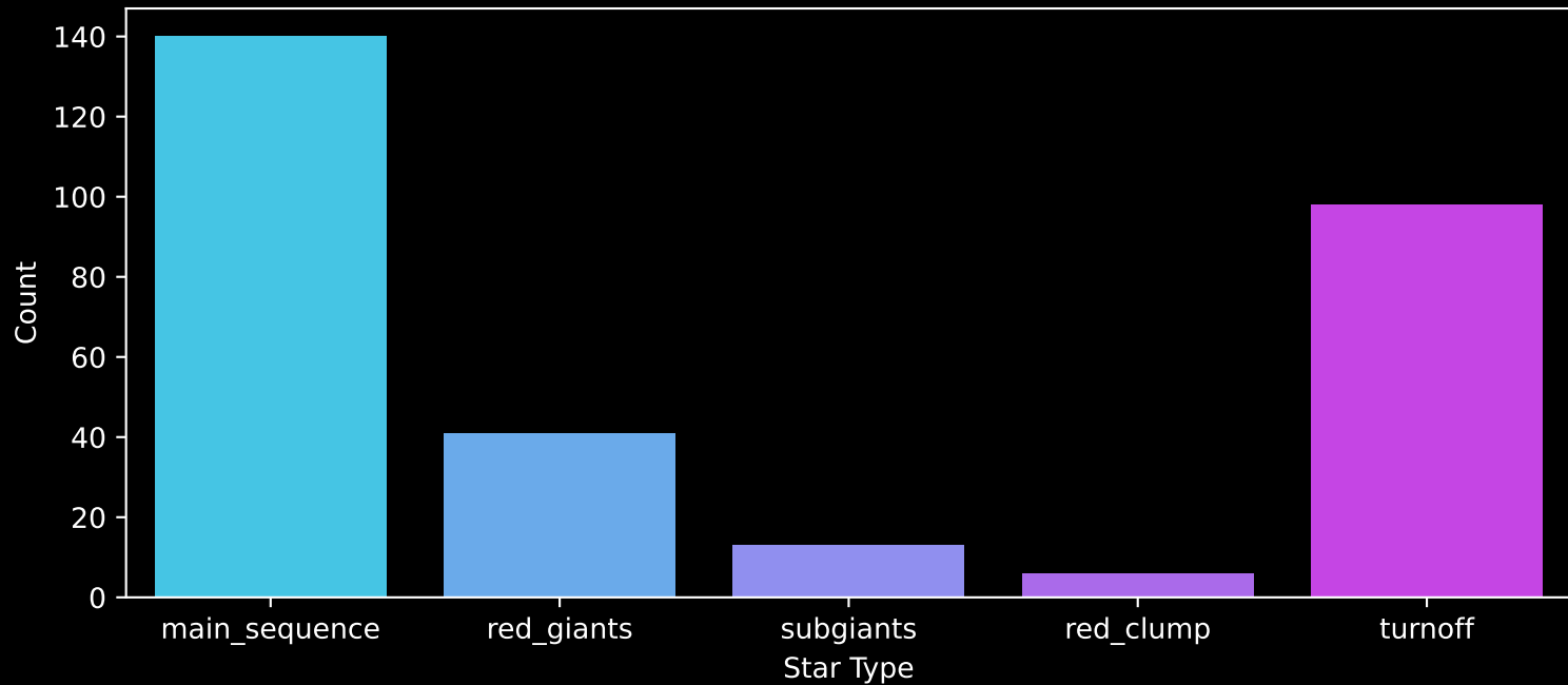
GALAH DR4 Field: [259] Count plot of Star Type
