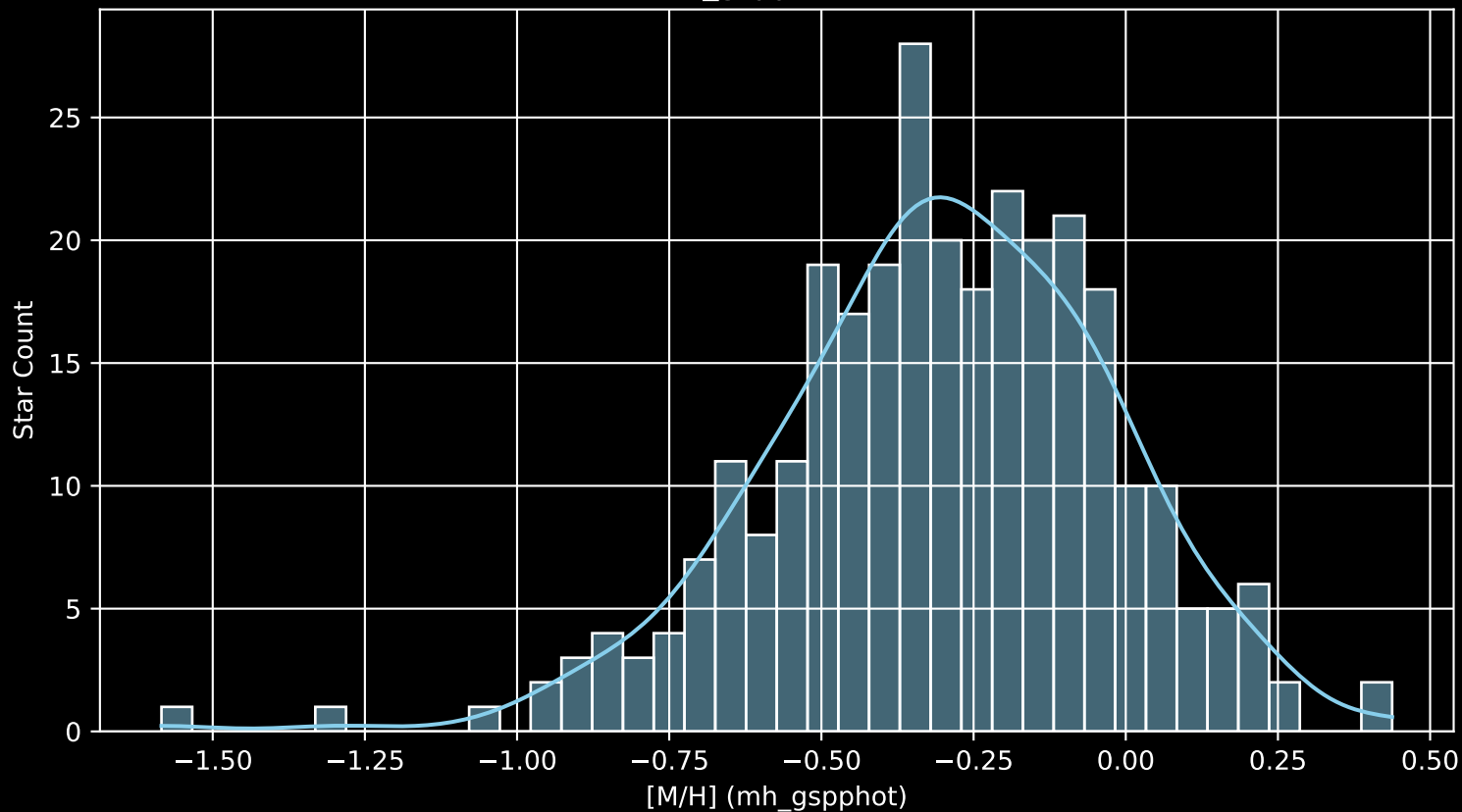
GALAH DR4 Field: [259] [M/H] (mh_gspphot) (n= 298)
