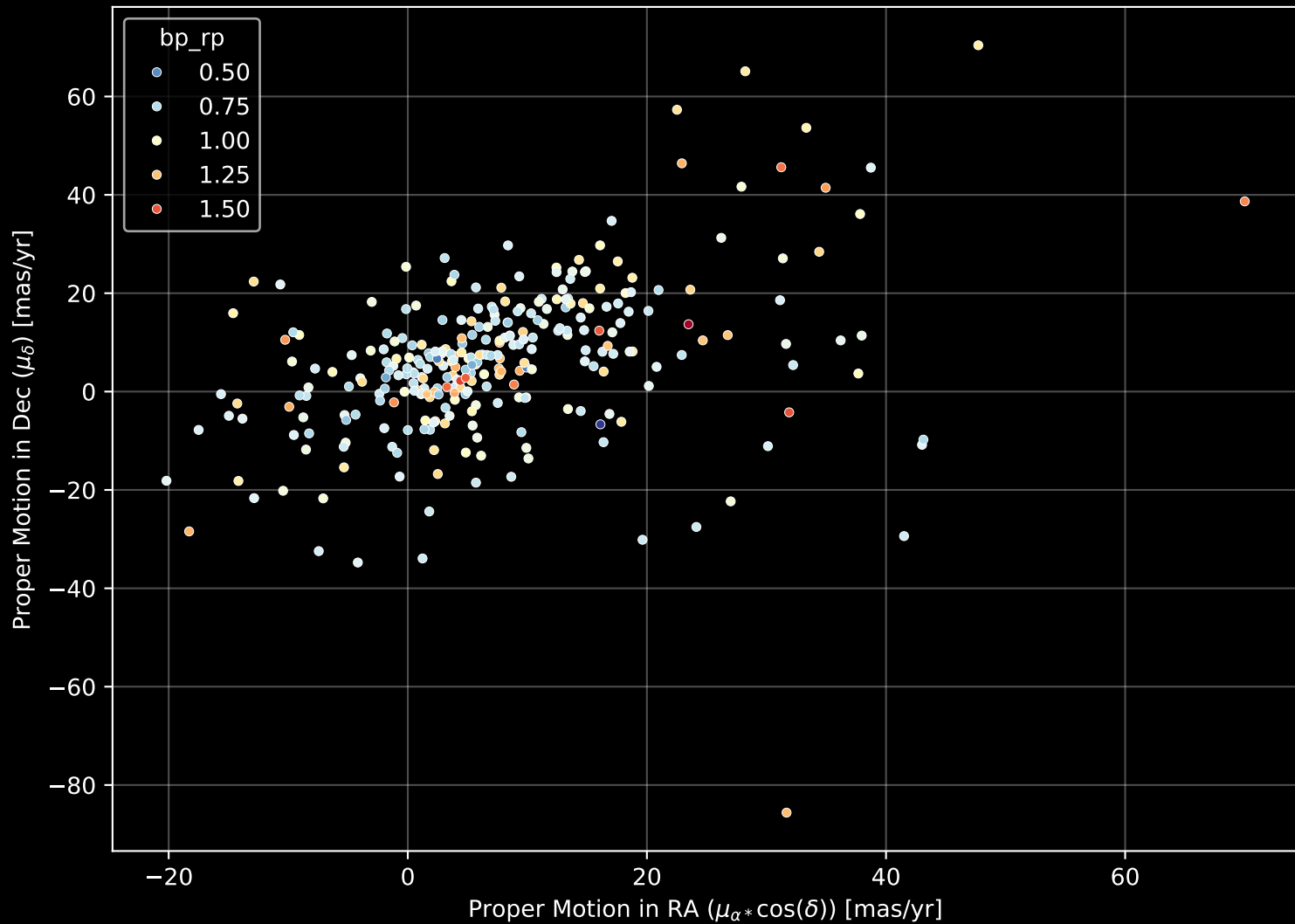
GALAH DR4 Field: [259] Proper Motion Diagram (n= 298)
