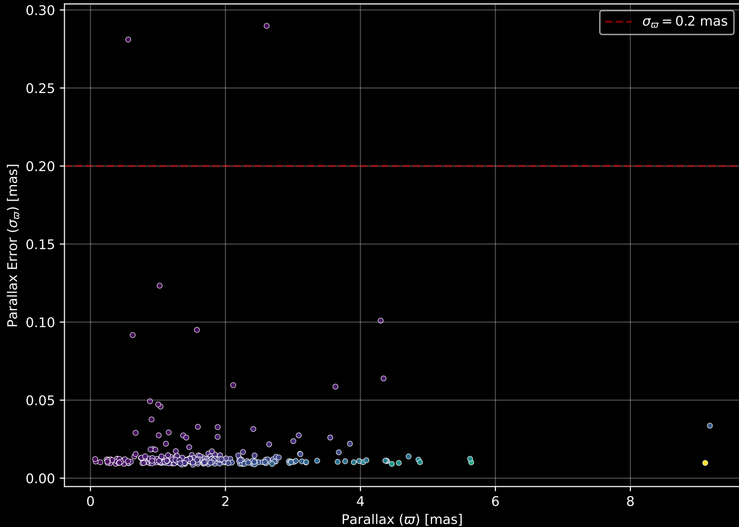
GALAH DR4 Field: [259] Parallax Quality (n= 298)
