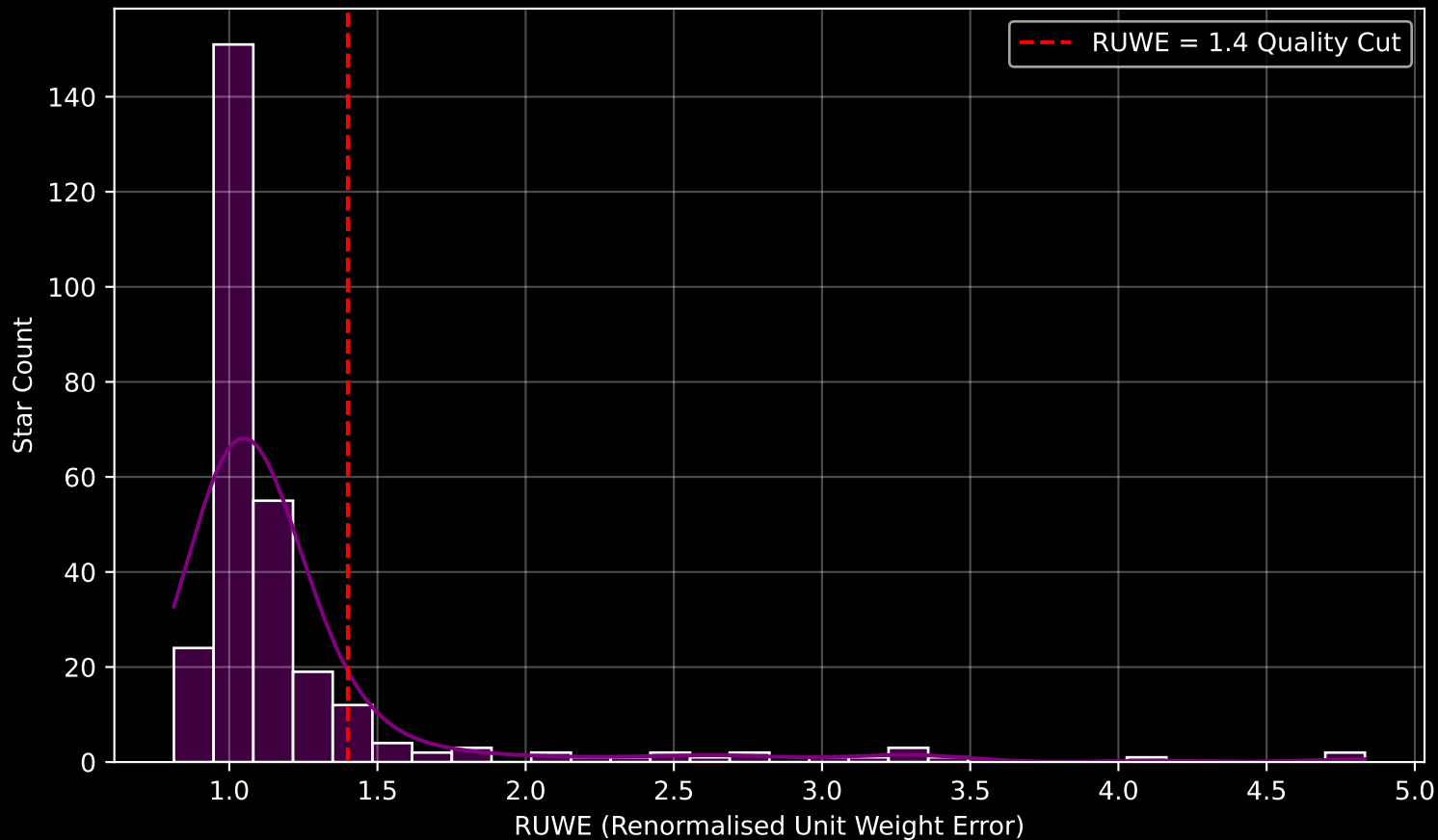
GALAH DR4 Field [259] RUWE Distribution (n= 288)
